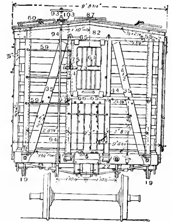
Fig. 370. End Elevation.
